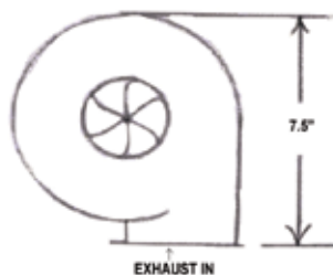
LARGEST EXHAUST HOUSING
